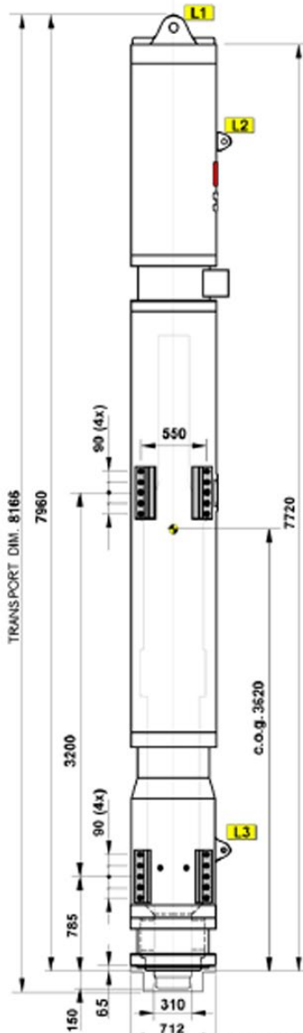
Main dimensions
