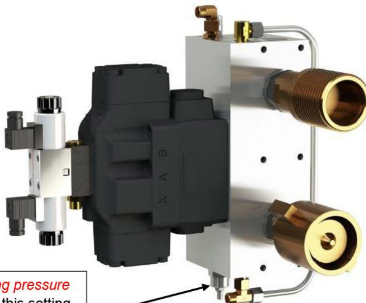
Figure 14 Auger manifold 1000693
