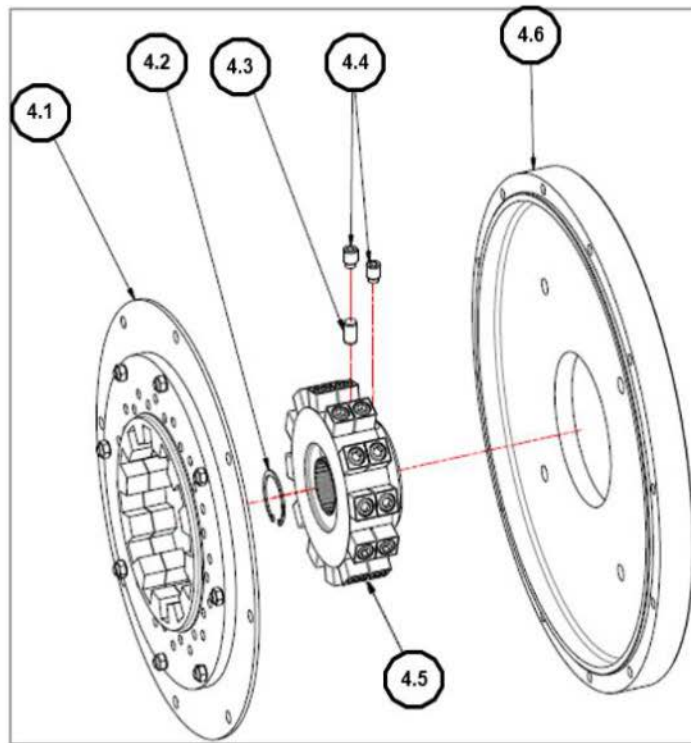
Figure 11 Motor/pump coupling
