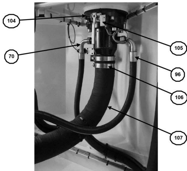
Figure 9 Intake manifold
