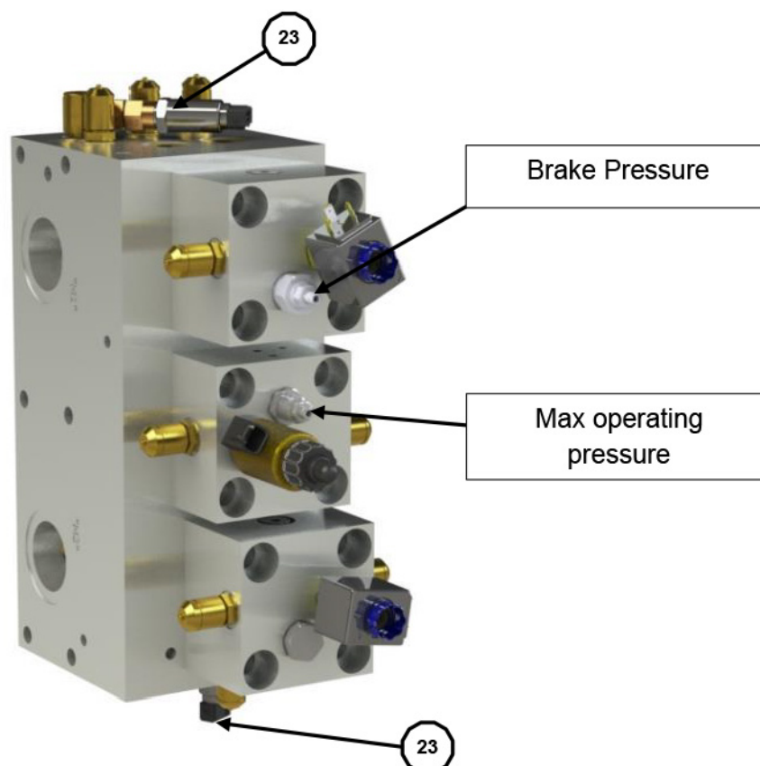
Figure 13 drive manifold 1000669
